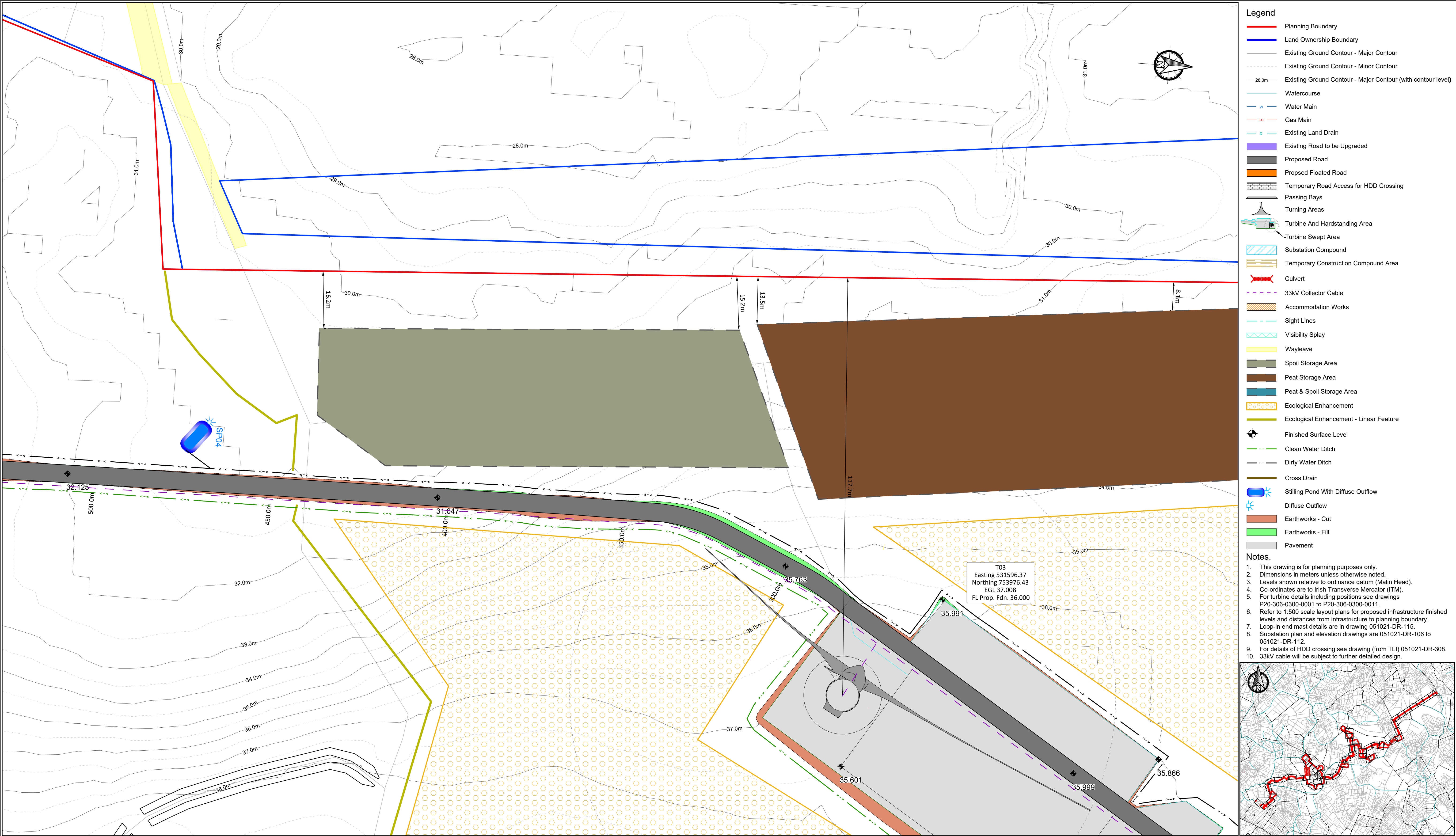
PLAN Scale 1:500 KEYPLAN Scale 1:80000
